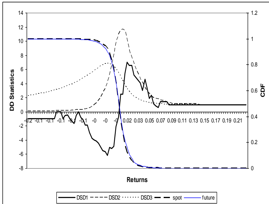
Figure 3: DCDFs of Returns for Spot and Futures and their Corresponding and DD Statistics for Risk Seekers
